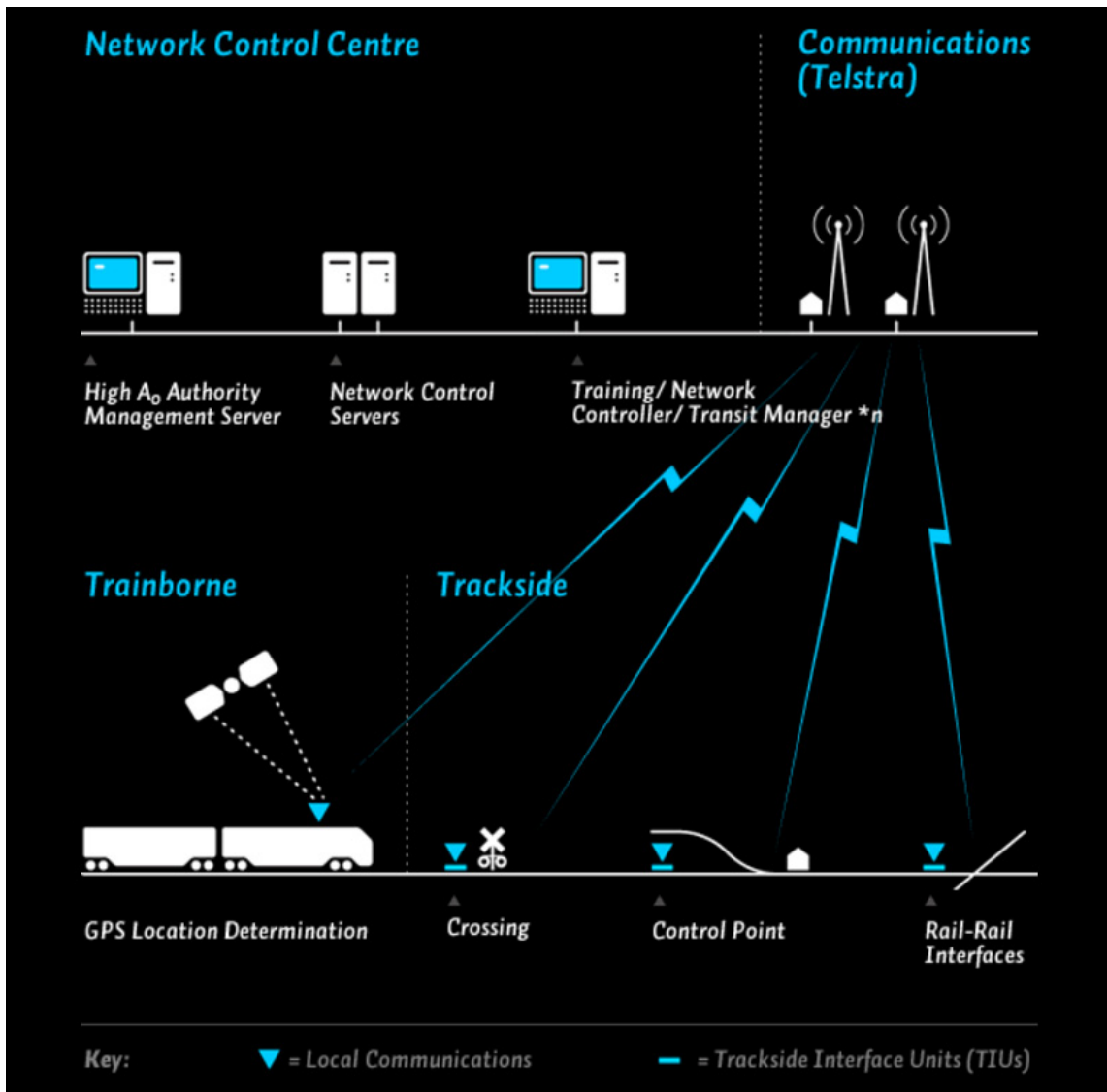
Figure 2-3 - ATMS architecture
