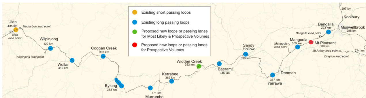
Figure 4-1 - Ulan Loops
