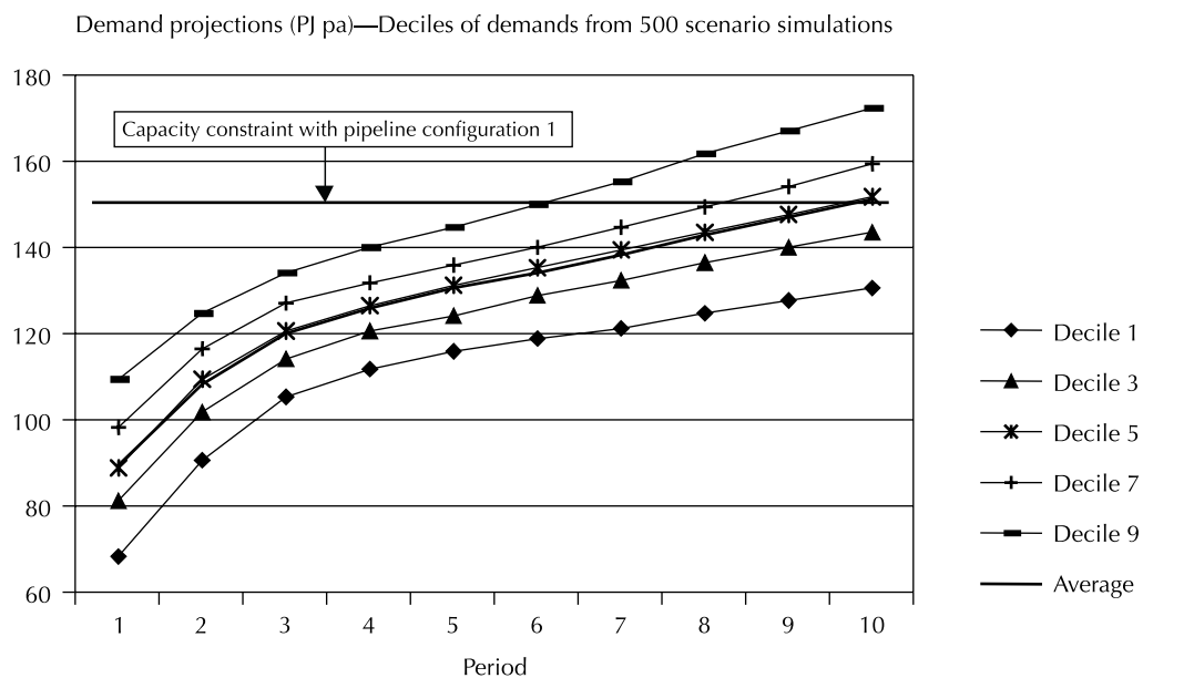
Graph A1.2. Selected deciles of demand in each year from 500 projection scenarios based on randomised parameter values
